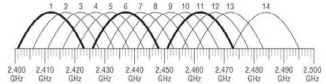
Figure 2: 20 MHz channels on the 2.4 GHz frequency band. 1
