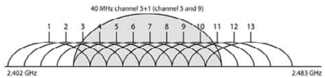
Figure 3: 40 MHz channels on the 2.4 GHz frequency band. 2
